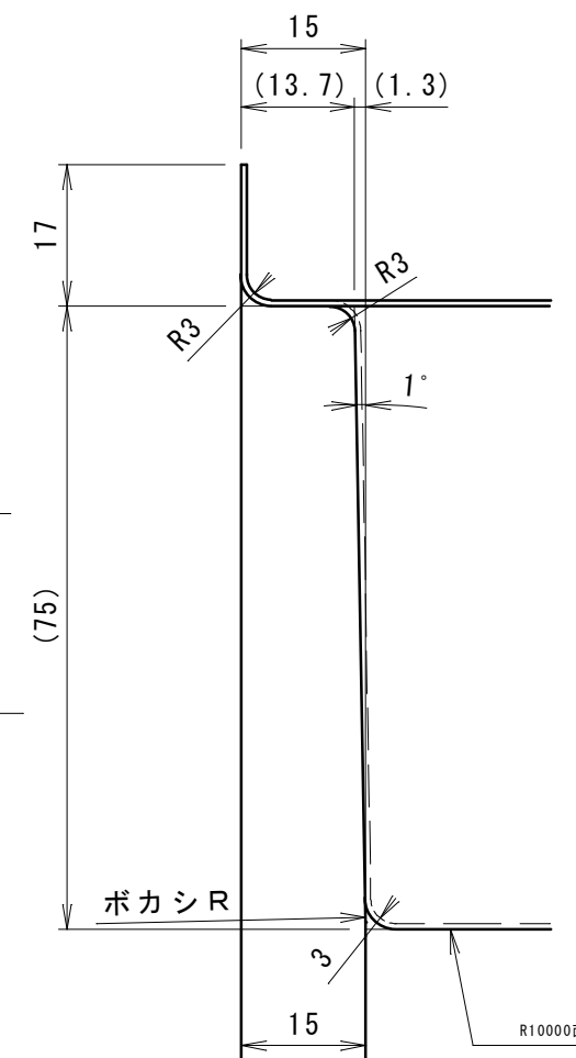
D 部詳細 (1/1)
