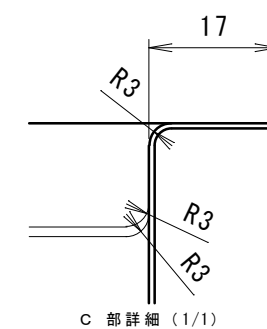
C 部詳細 (1/1)
